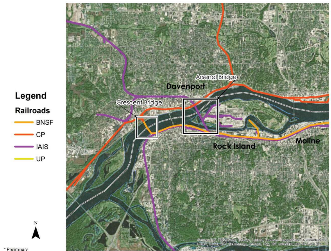
Figure 3.20 Study Area Railroad Bridges
