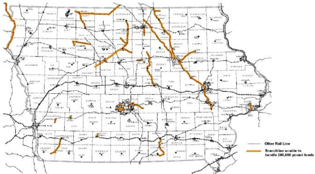
Figure 5.6 Track-Miles Unable to Handle 286,000 Pound Rail Cars
